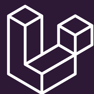
Laravel
