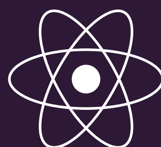
React
